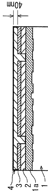
FIG. 22F Form hole injection layer
